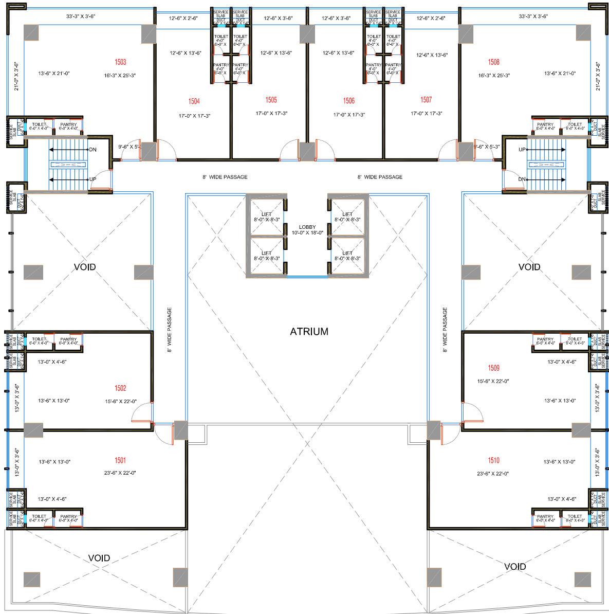
15TH FLOOR PLAN OF TWO WINGS
