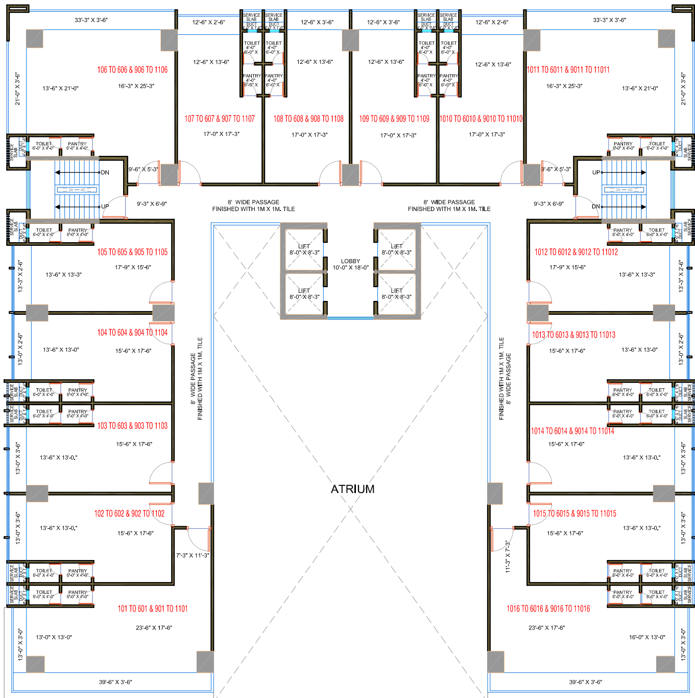
TYPICAL FLOOR PLAN FROM 1ST TO 6TH, 9TH TO 11TH OF TWO WINGS
