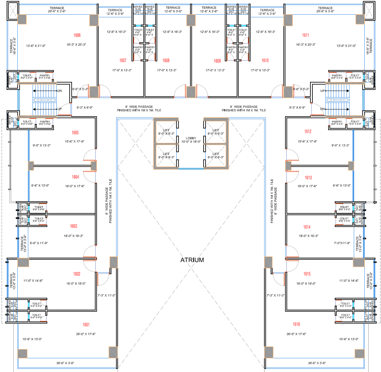
16TH FLOOR PLAN OF TWO WINGS
