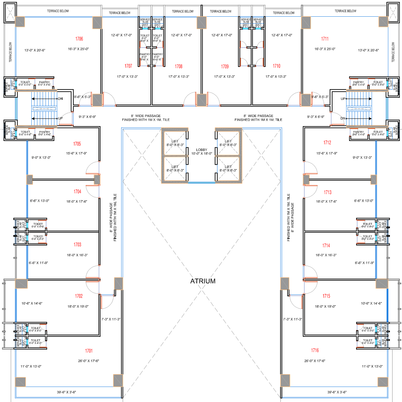
17TH FLOOR PLAN OF TWO WINGS
