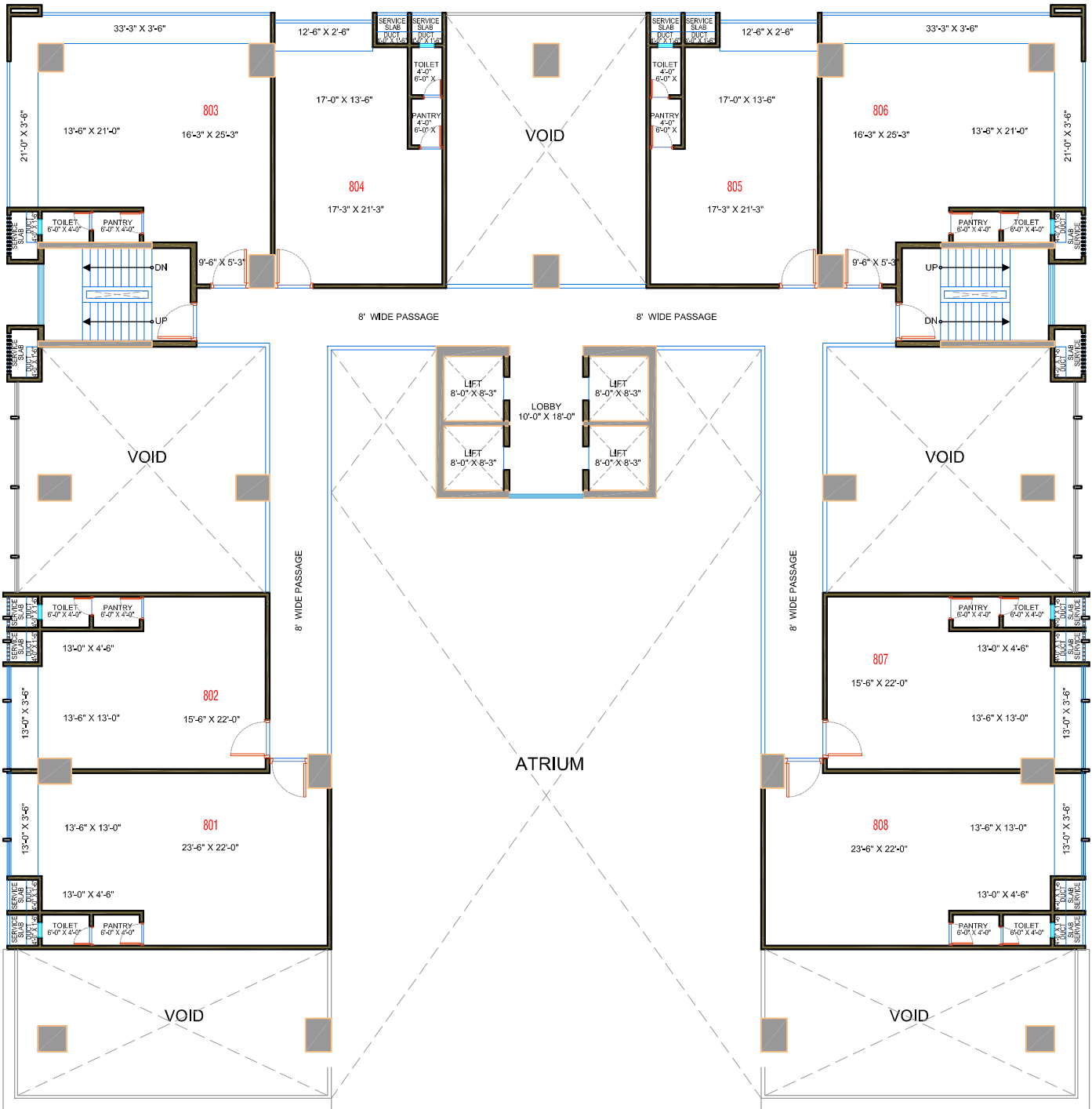
8TH FLOOR PLAN OF TWO WINGS
